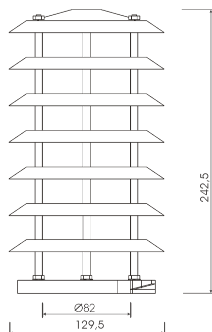
Big stainless steel louvre reflector mounted upwards
