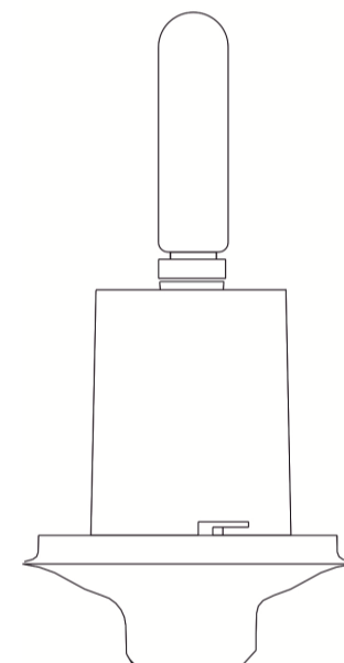
Mounting of the stainless steel louvre reflector in the luminaire E-40
