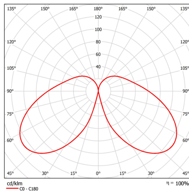
Distribution curve KARIN 1200 LED
