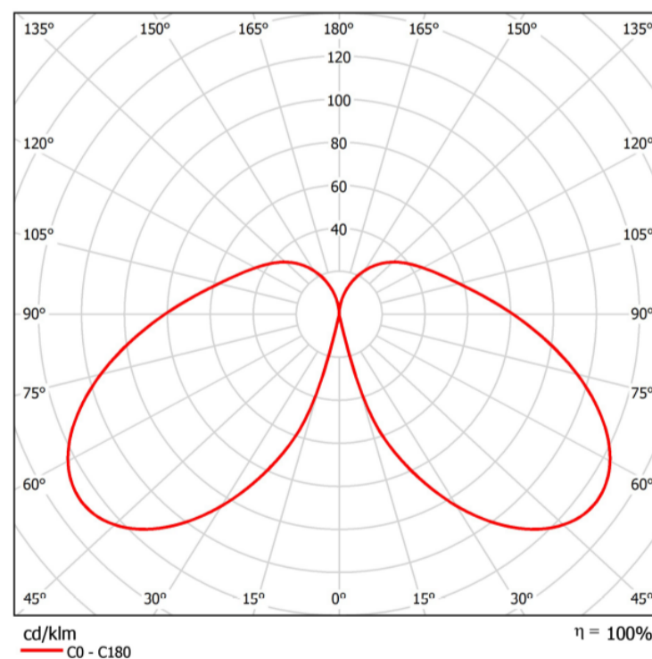
Distribution curve KARIN 600 LED
