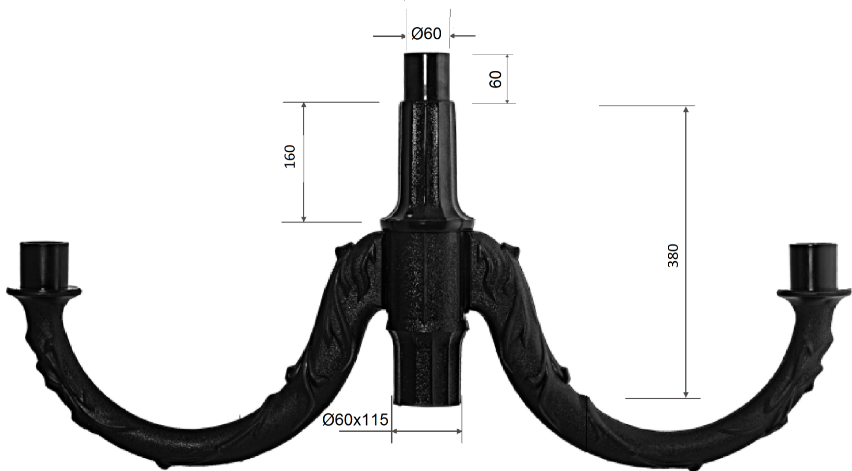
Arm system „2+1” upwards
